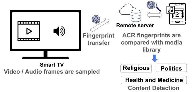
Figure 1: ACR system architecture: fingerprint capture, transmission, and content detection.
