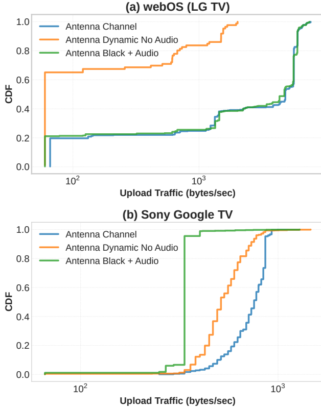
Figure 6: CDF of Antenna sub-scenarios on webOS (LG TV) and Sony Google TV. The x-axis shows the upload traffic rate to the ACR endpoint; the y-axis shows cumulative fraction of seconds with traffic rate \leq x . webOS employs audio-based ACR: “Antenna Dynamic No Audio” shows a 97.3% mean traffic reduction, while “Antenna Black + Audio” shows no decrease. Samba TV ACR on Sony Google TV employs video-based ACR: “Antenna Dynamic No Audio” produces high periodic traffic, whereas “Antenna Black + Audio” results in a 52.9% mean reduction.
