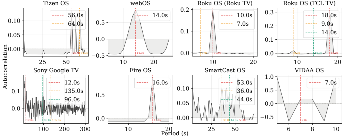
Figure 5: Autocorrelation of upload traffic for identified ACR endpoints. The x-axis shows the lag in seconds and the y-axis shows the normalized autocorrelation coefficient; a strong peak at lag T indicates that the traffic repeats with period T . Dashed vertical lines mark the top-3 dominant periods detected per OS. All endpoints exhibit clear periodic behavior, with dominant periods ranging from 7 seconds (VIDAA OS) to approximately 135 seconds (Sony Google TV). This periodicity supports our hypothesis that ACR implementations transmit fingerprints at regular intervals for real-time content identification (§5.1).
