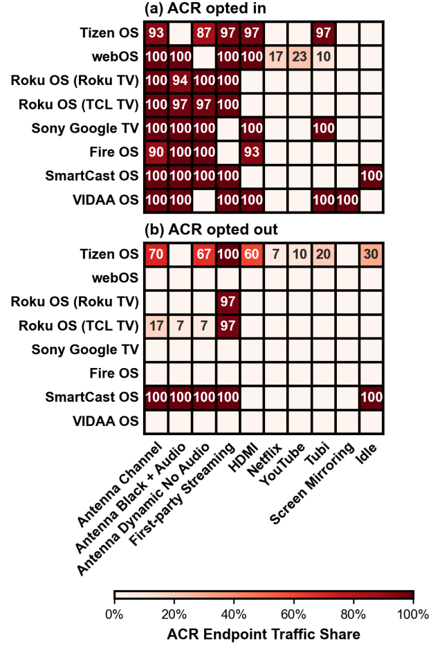
Figure 7: Share of measurements (out of 30) in which the identified ACR endpoint received content-correlated traffic, per TV and scenario, in the opted-in (top) and opted-out (bottom) states. The opted-in panel shows the bimodality our classification thresholds rely on: scenarios cluster near 100% or near 0% with no ambiguous cases. The opted-out panel shows opt-out effectiveness: cells that remain dark indicate persistent traffic after opt-out. Plaintext ACR data is accessible on VIDAA OS and a single-measurement analysis is sufficient to characterize ACR-subject scenarios.
