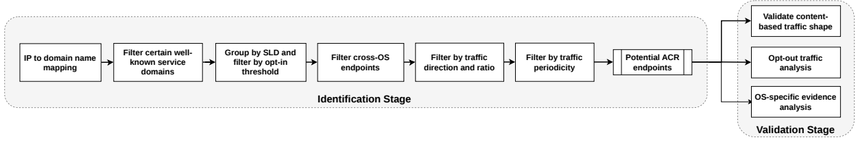
Figure 3: ACR endpoint identification and validation. The identification stage filters each TV’s destination set to candidate endpoints through well-known service domain removal, opt-in-frequency threshold, cross-OS filtering, and traffic-direction and periodicity tests. The validation stage corroborates each candidate against content-modality response, opt-out behavior, and OS-specific evidence.
