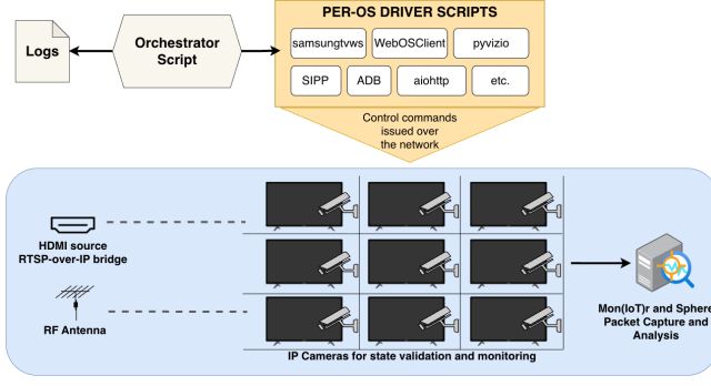
Figure 2: Data collection infrastructure. The orchestrator dispatches per-OS driver scripts over Wi-Fi while Mon(Io)Tr and SPHERE Research Infrastructure software captures all TV-originated traffic at a gateway. An RTSP-to-HDMI bridge supplies controlled HDMI content; an HDMI-to-RF modulator supplies controlled antenna stimuli; per-TV IP cameras record on-screen state for per-trial validation.
